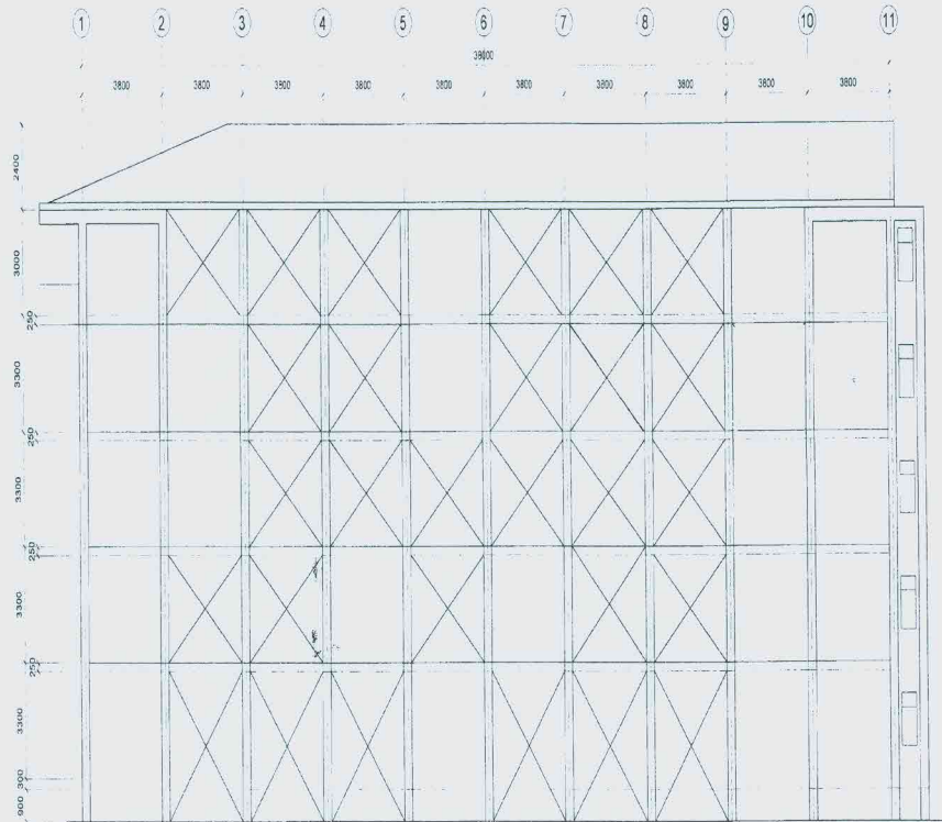
LAYOUT OF CROSS BRACINGS (FRONT ELEVATION)
